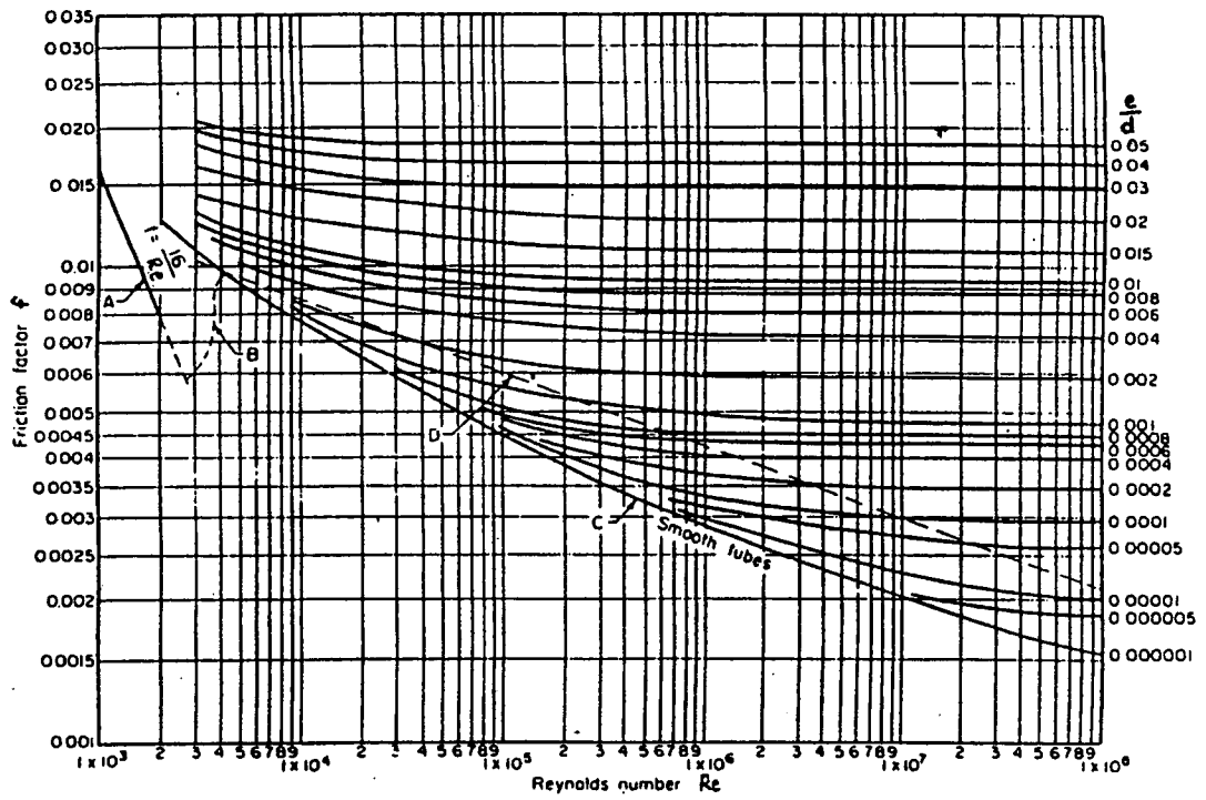
Figure 1. Moody chart
