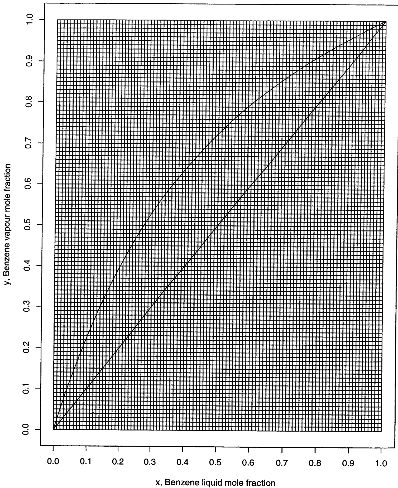
Figure 2: Benzene/Chlorobenzene Equilibrium curve
