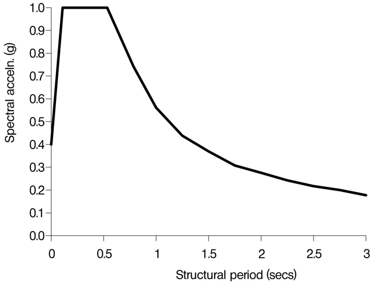
FIGURE Q8-2 : 475 year return period 5% damped spectrum for the region for rock with a wave velocity V_s of at least 2625 ft/s at the surface
