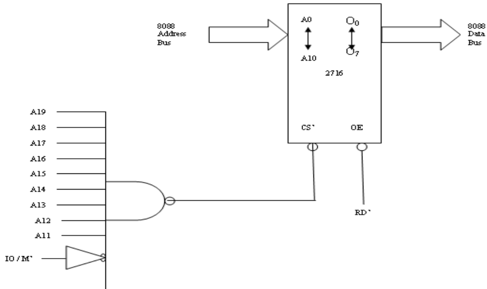
A simple NAND gate decoder used to select a 2716 EPROM
