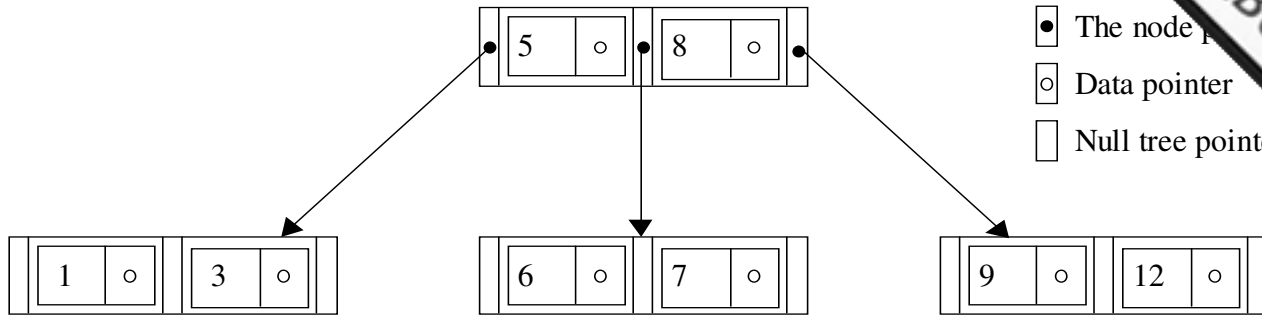
An index structure for B-tree
