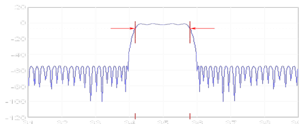
Figure 1: A graph of a bandpass filter's gain magnitude, illustrating the concept of -3 dB (or half-power) bandwidth
