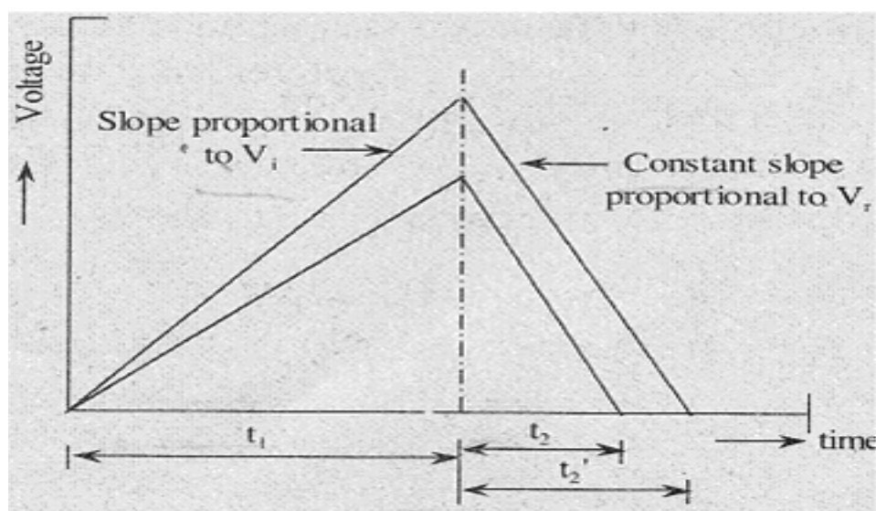
fig. 5. a. (ii) Basic Principle
