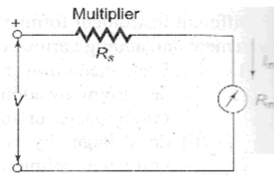
fig 4.a. (i) Basic Voltmeter
