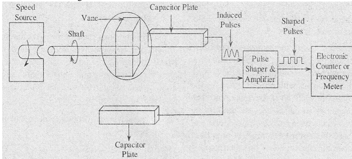
fig 8.b. Capacitive Transducer
