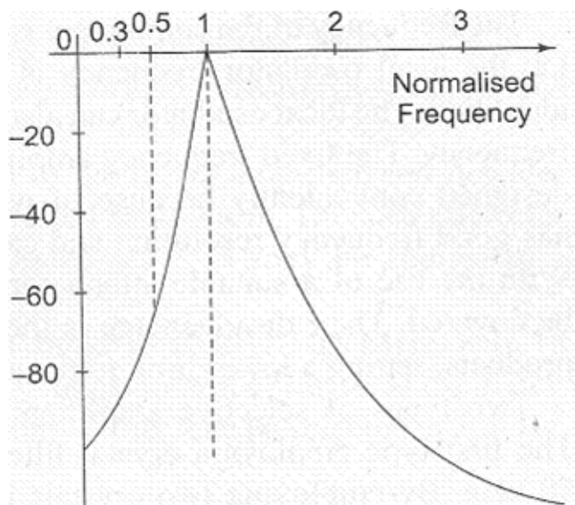
fig7.a.(ii) Relative response in db
