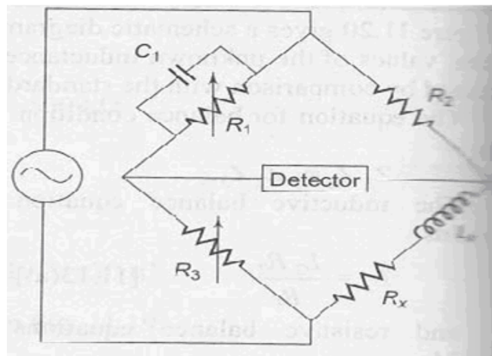
Maxwell's Bridge
