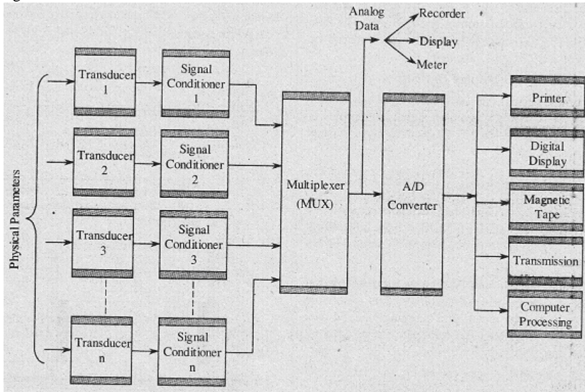
fig.9.b. Generalised Data Acquisition System
