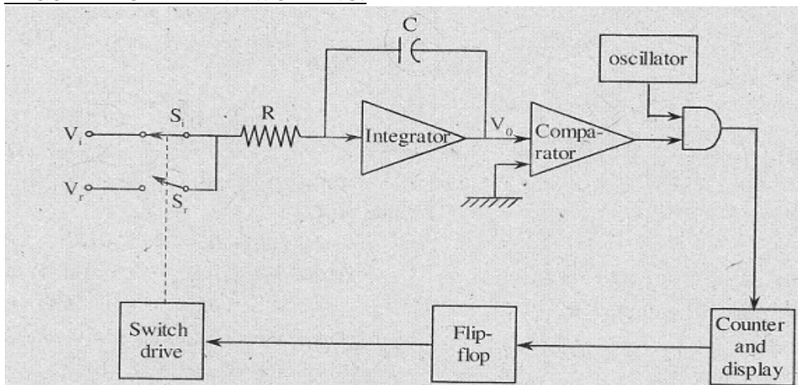
fig. 5. a. Block Diagram of Dual Slope integrating Type DVM
