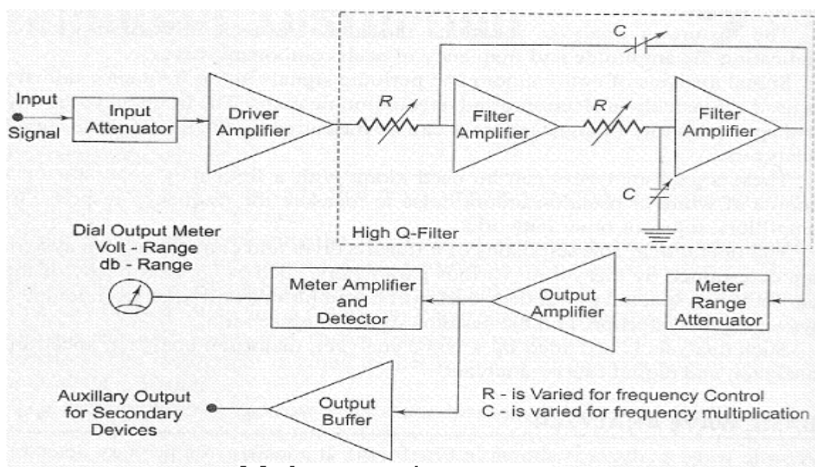
fig.7.a. frequency wave analyser
