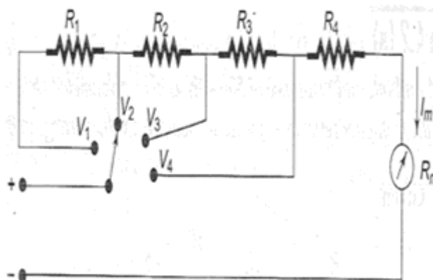
fig 4. a. (ii) Multiplier Connected in Series String
