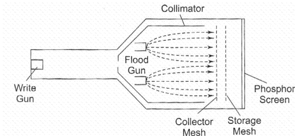
fig6.b.(ii) Storage mesh CRT
