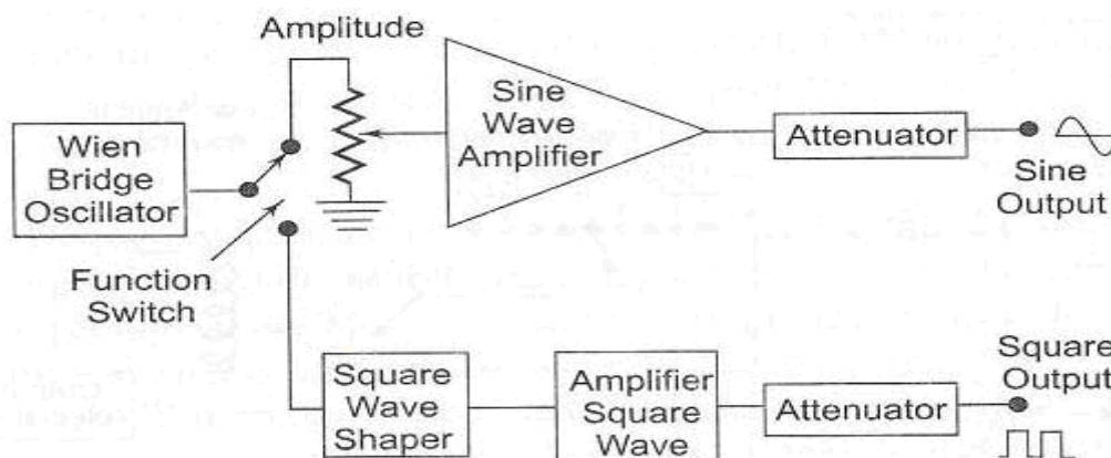
fig.6.a.(ii) AF sine &amp; Square wave generator
