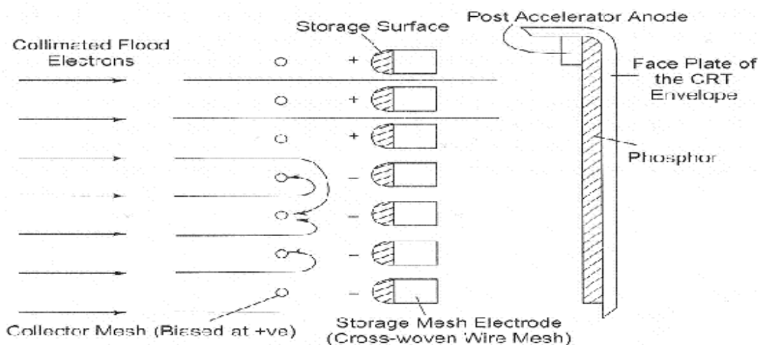
fig6.b.(iii) Display of stored charge pattern on mesh
