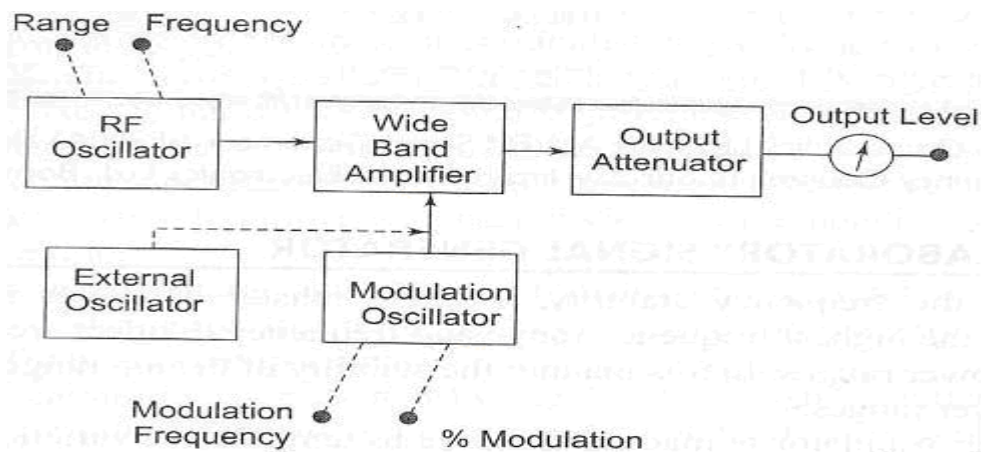
fig.6.a. conventional Signal generator
