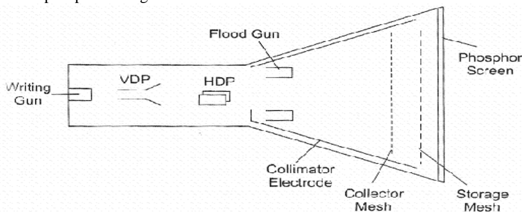
fig 6.b Basic Elements of storage mesh CRT
