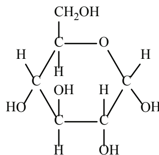
Molecule 3
