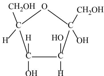
Molecule 5
