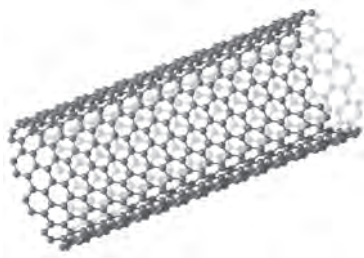
carbon nanotube
