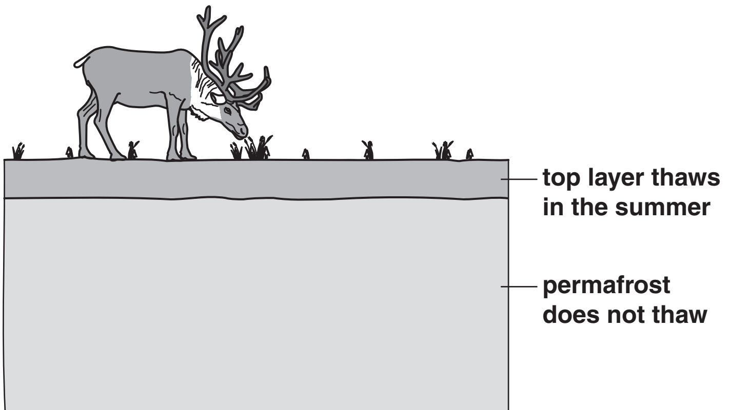
section through Arctic soil
