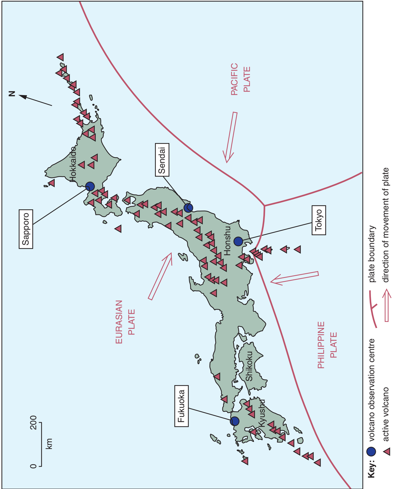
Fig. 8 Active volcanoes in Japan
