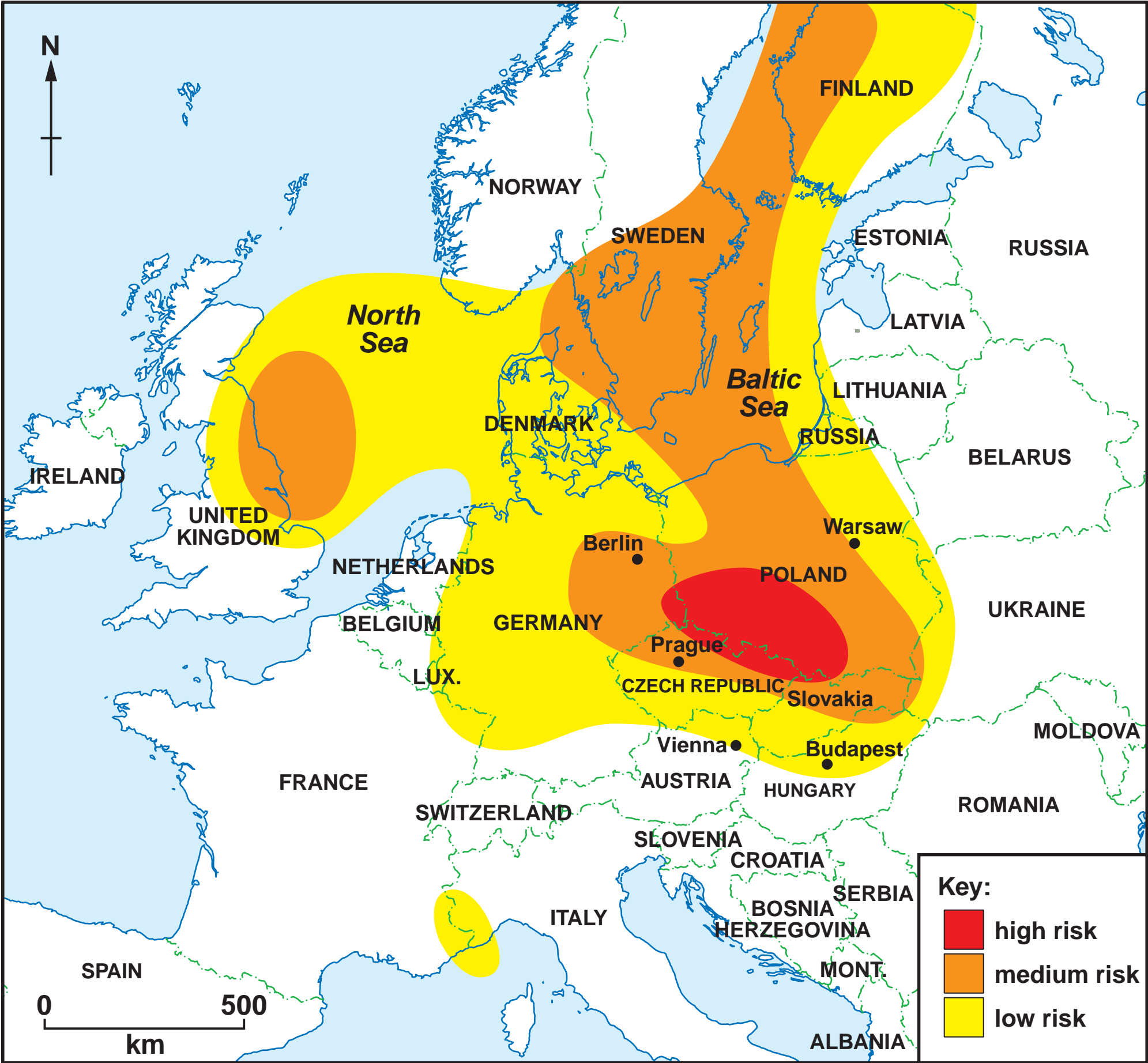
MAP J ACID RAIN IN EUROPE
