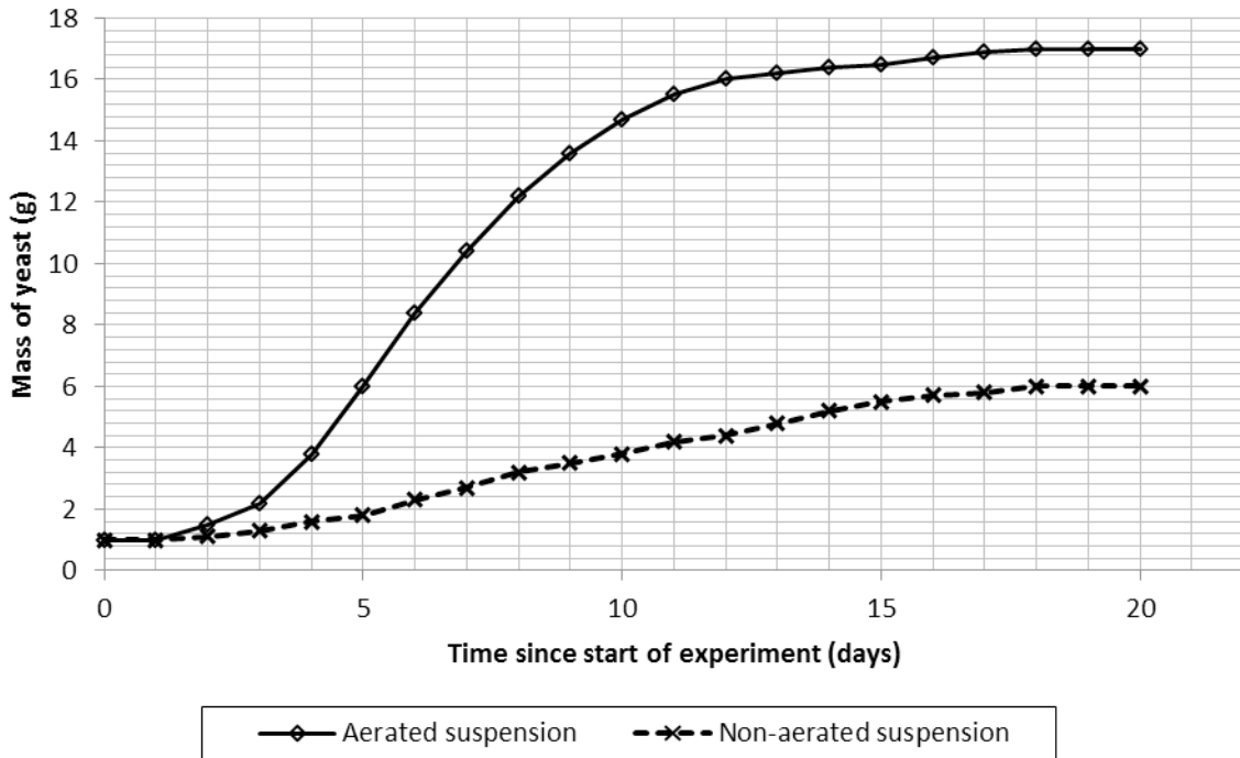
Effect of aeration on yeast growth
