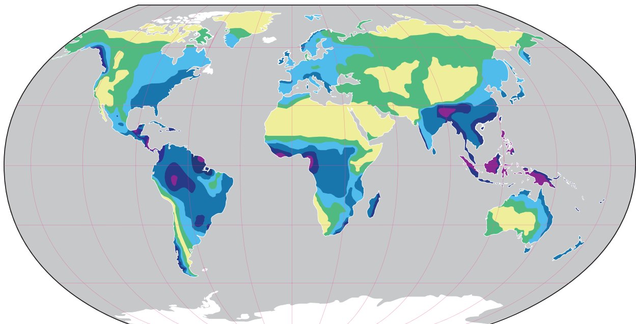
Figure 9: The global rainfall pattern
