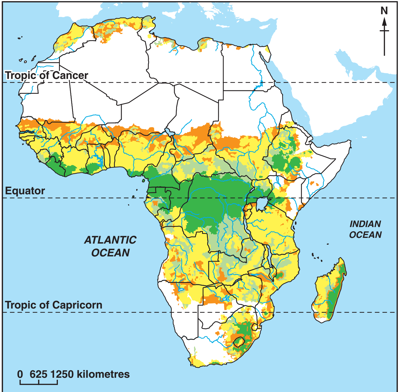
FIG. 4 AREAS OF AFRICA AT RISK OF DESERTIFICATION
