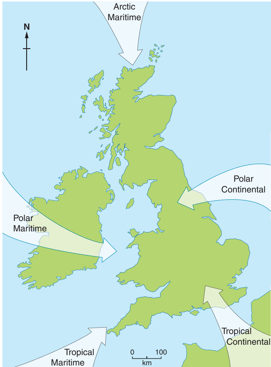
Fig. 1 The main air masses affecting the British Isles
