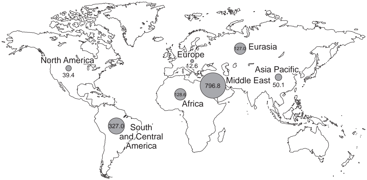
World distribution of oil reserves, 2011
