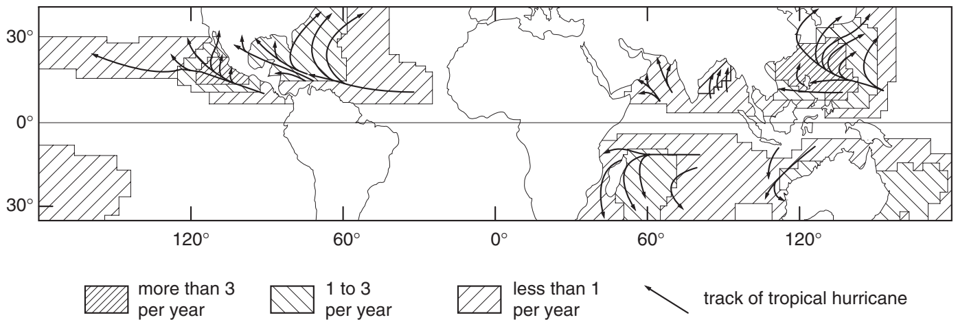
Tropical storm (hurricane) events in the tropics
