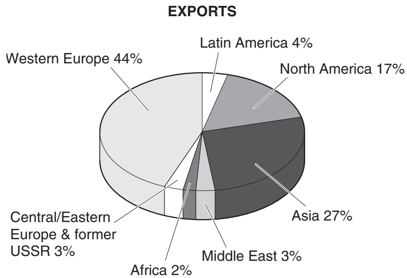
Percentage value of global imports and exports in 1994
