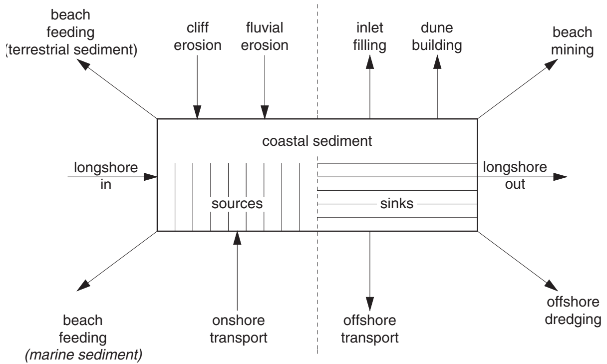
Sources and sinks of coastal sediment within a sediment cell
