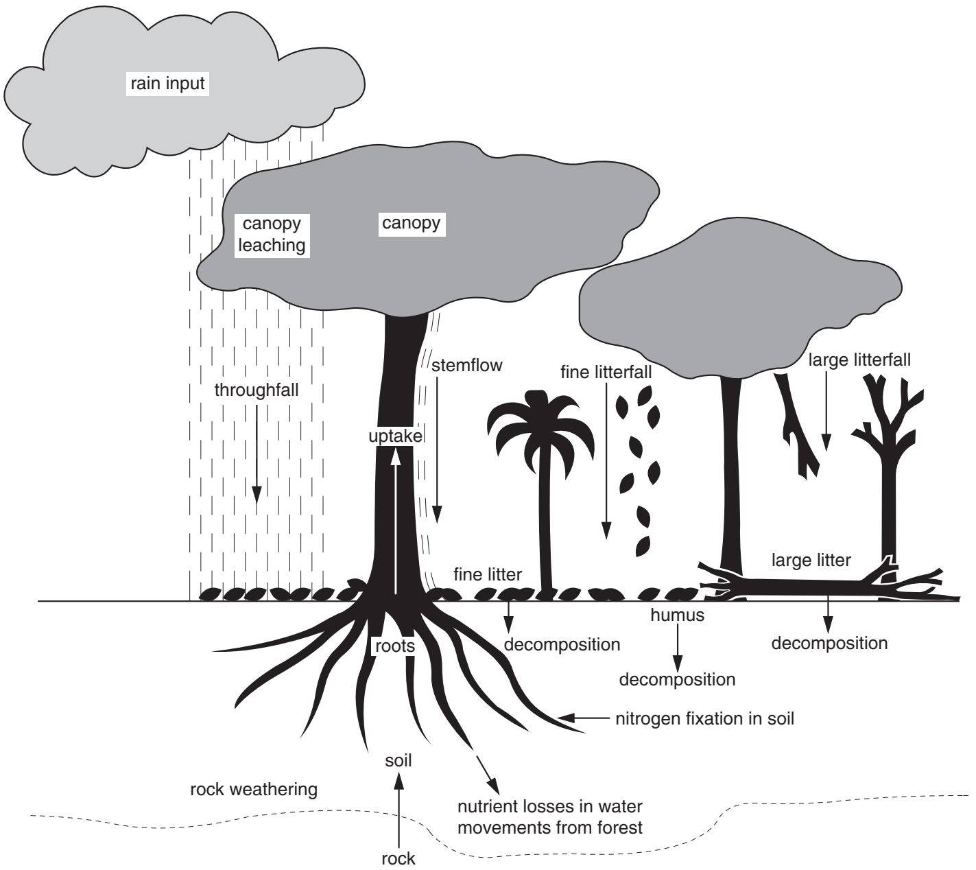
Nutrient flows and stores in the tropical rainforest
