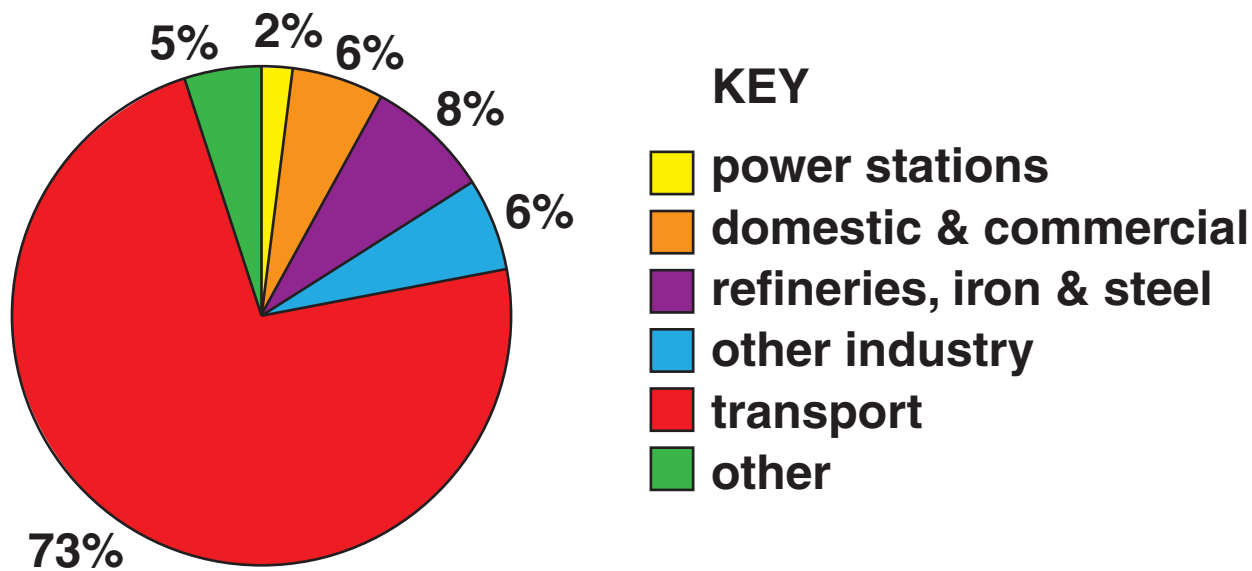
Fig. 3 Sources of Carbon Monoxide Pollution in the UK
