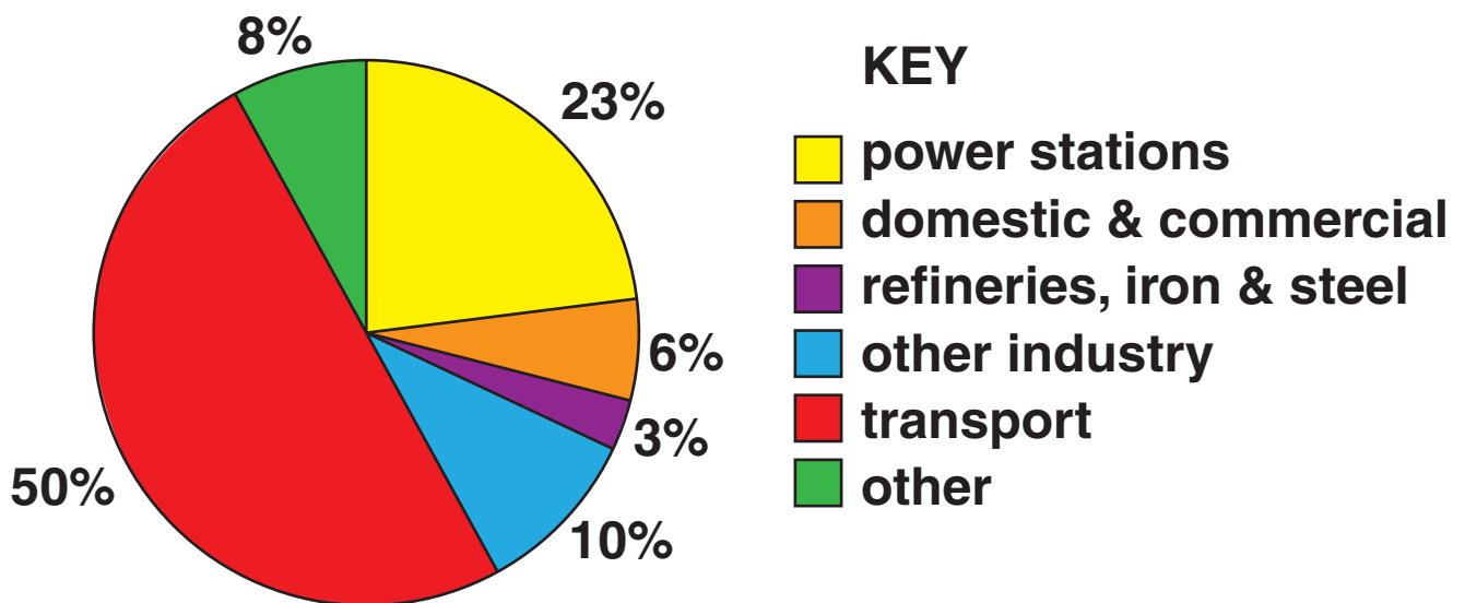
Fig. 2 Sources of Nitrogen Oxides Pollution in the UK
