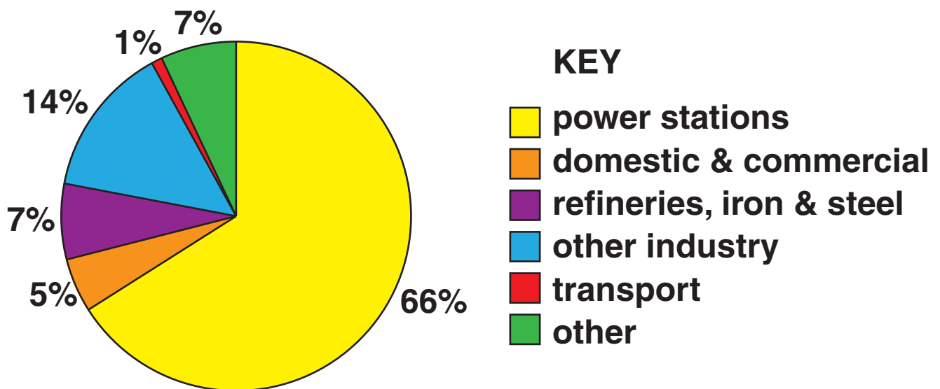
Fig. 1 Sources of Sulphur Dioxide Pollution in the UK
