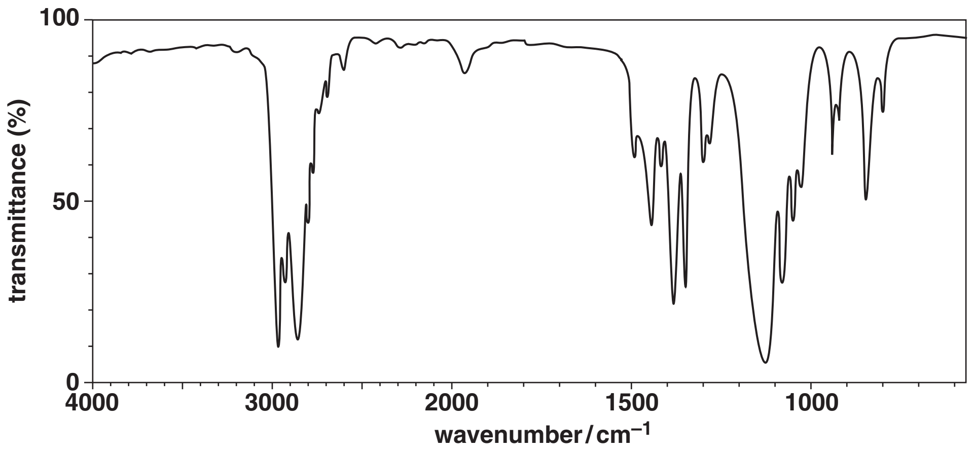
infrared spectrum of COMPOUND A
