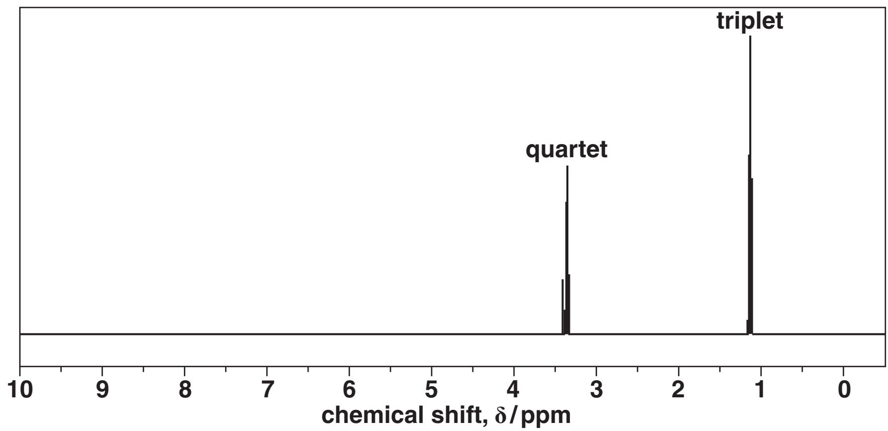
proton NMR spectrum of COMPOUND A
