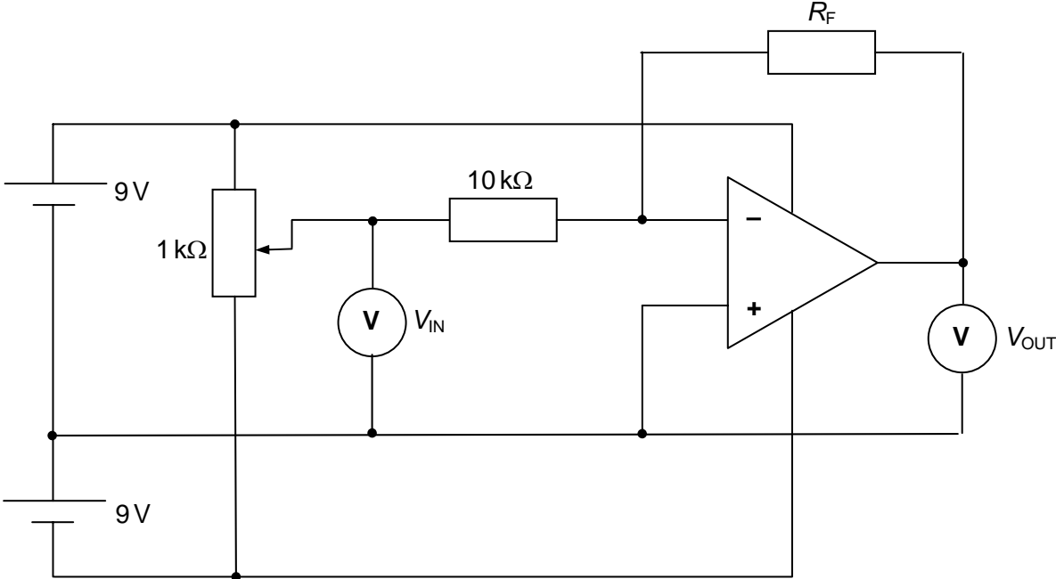
Circuit diagram for the inverting amplifier.
