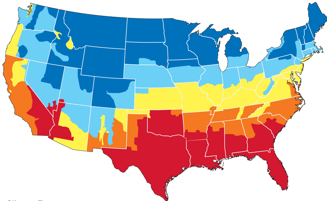
Figure 11: Variations in heating and cooling requirements in mainland USA, 1960–2010
