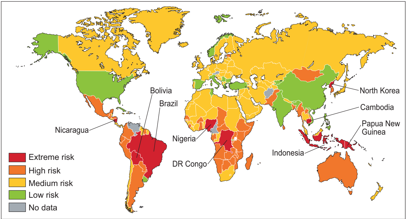
Figure 20: Areas where biofuel production increased the risk of deforestation in 2012
