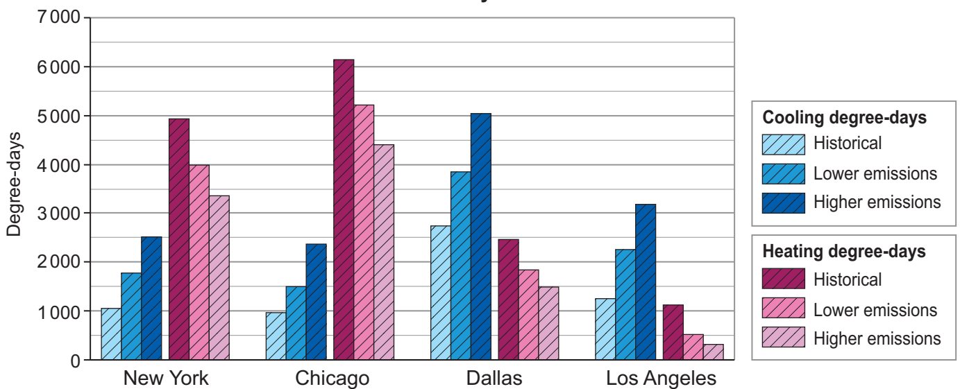
Figure 12: Predicted changes in heating and cooling degree-days for selected cities by 2080
