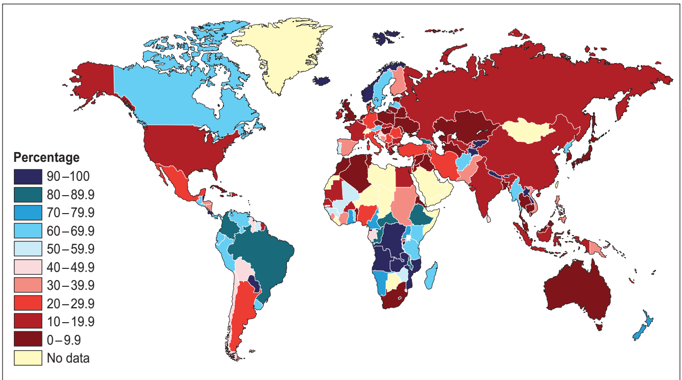
Figure 18: Percentage of electrical energy produced from alternative sources, 2012
