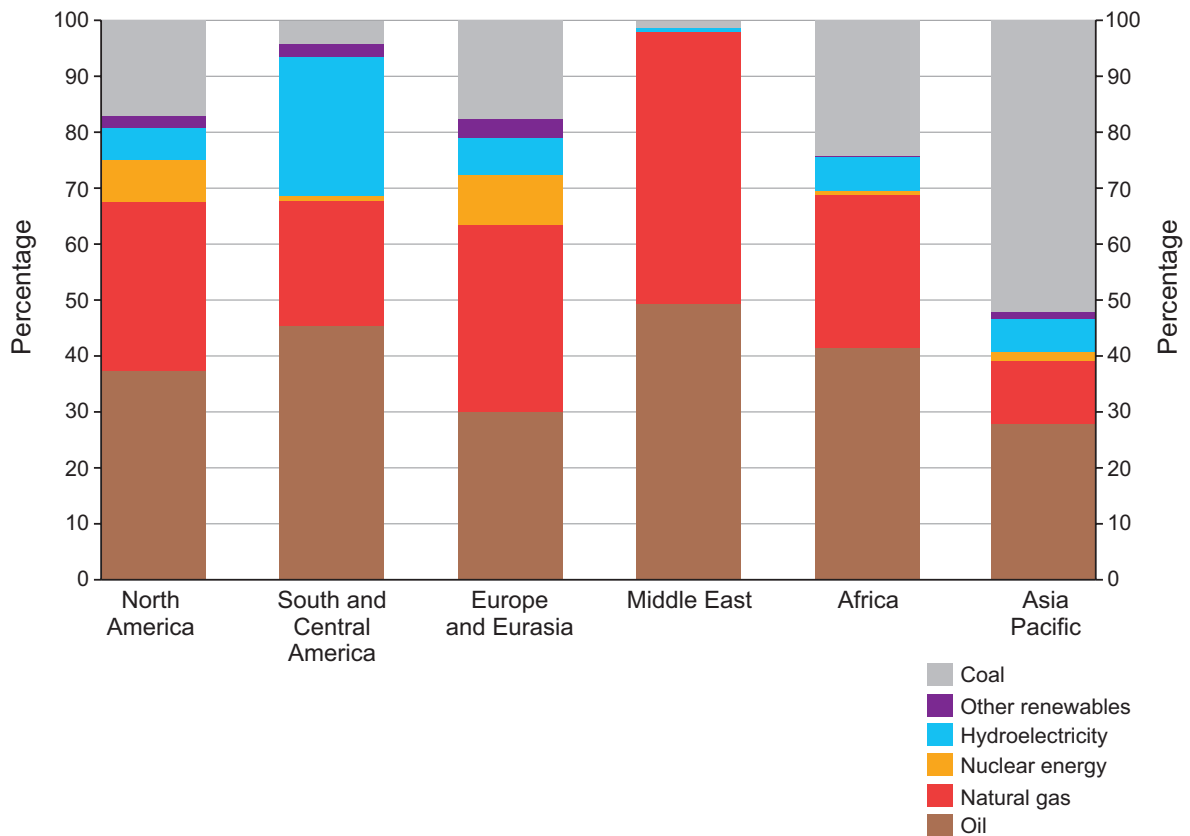
Figure 16: The energy consumption mix of world regions, 2012
