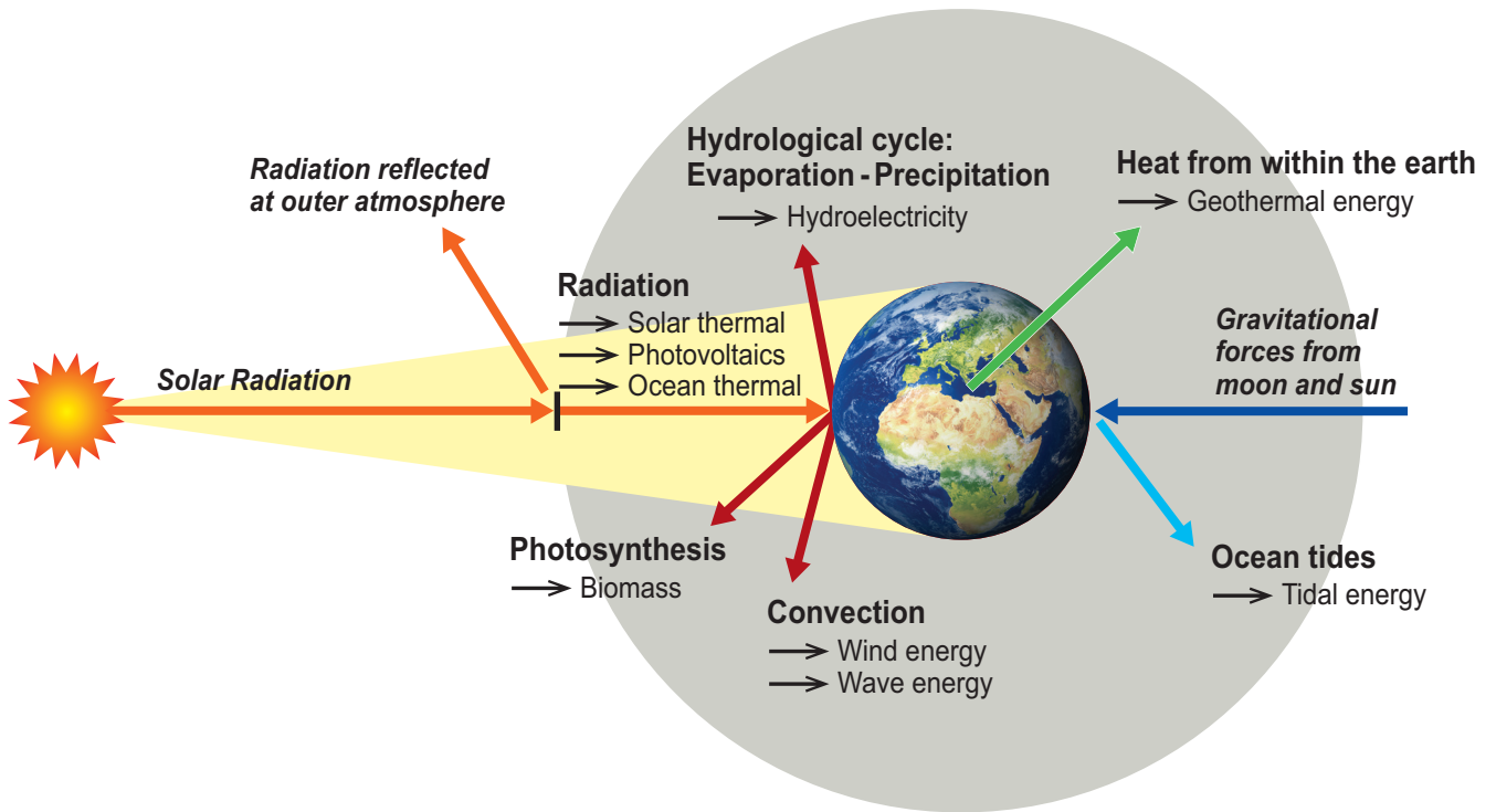
Figure 17: Alternative sources of energy
