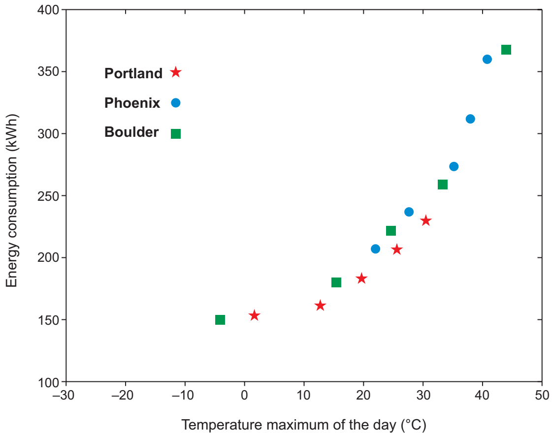
Figure 9: Relationship between temperature and energy consumption in supermarkets in three cities in the USA
