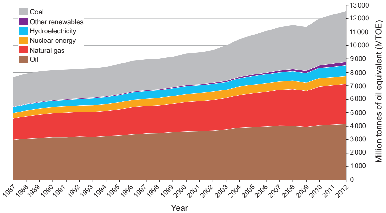
Figure 15: Global growth of energy consumption by source, 1987–2012
