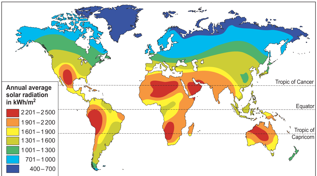
Figure 21: World solar energy potential
