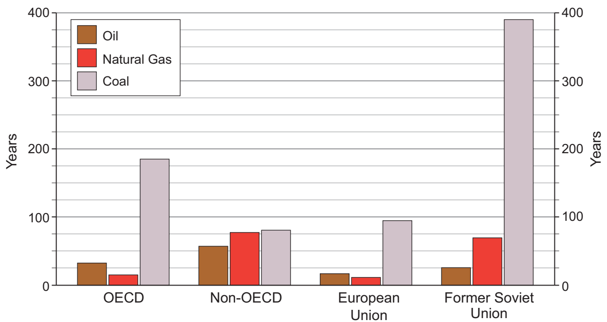
Figure 14: Expected number of years of indigenous fossil fuels available after 2012 in selected regions
