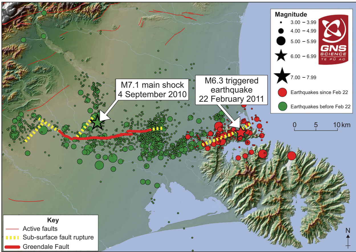
Figure P8 – Earthquake epicentres in the Christchurch region: September 2010–May 2011
