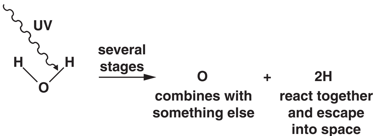
FIG. 1 Ultraviolet dissociation of water
