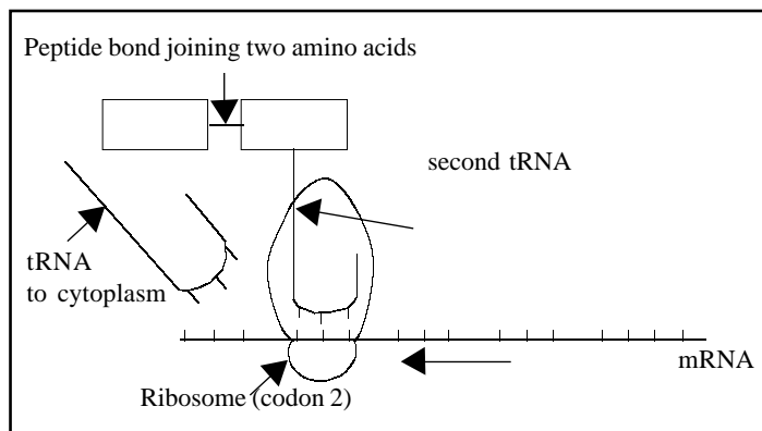
Fig 6. Translation Step 2
