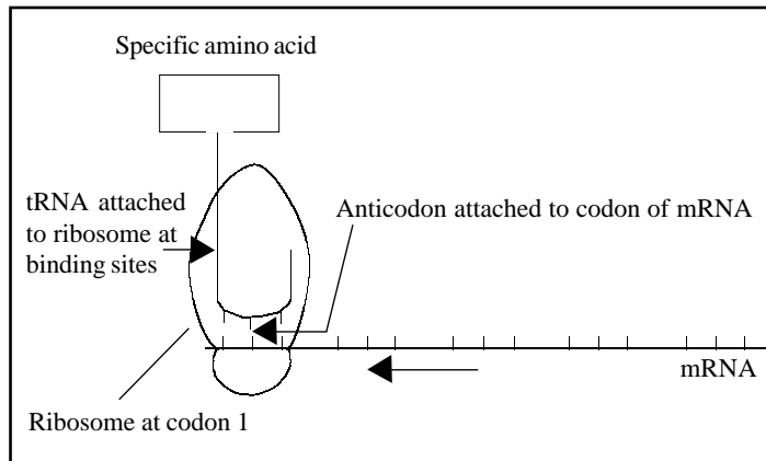
Fig 5. Translation Step 1
